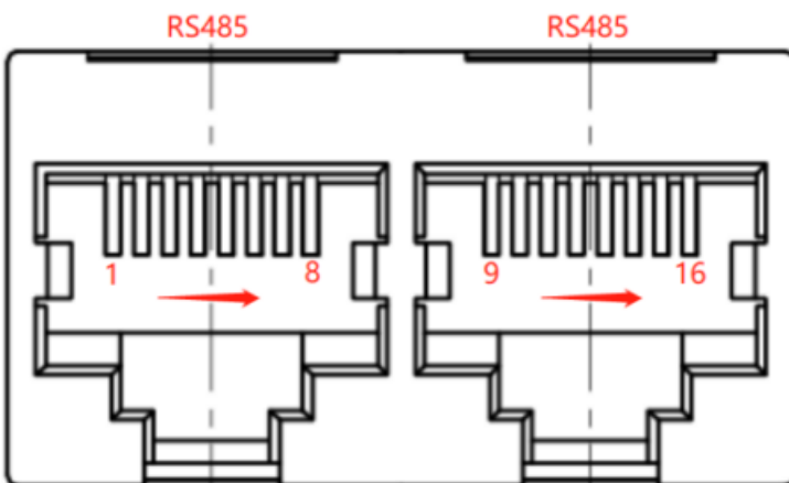
Parallel communication port
